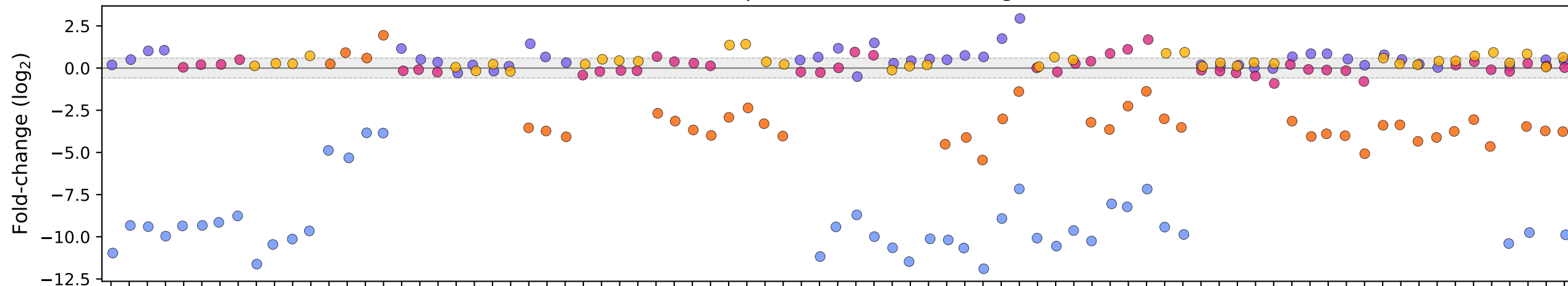
C) Biomass vs. metabarcoding reads
