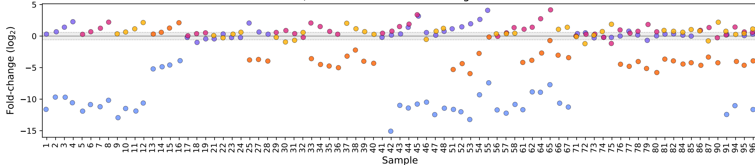
C) Biomass vs. metabarcoding reads
