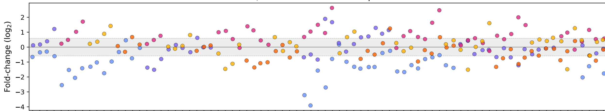
B) mtDNA copies vs. metabarcoding reads
